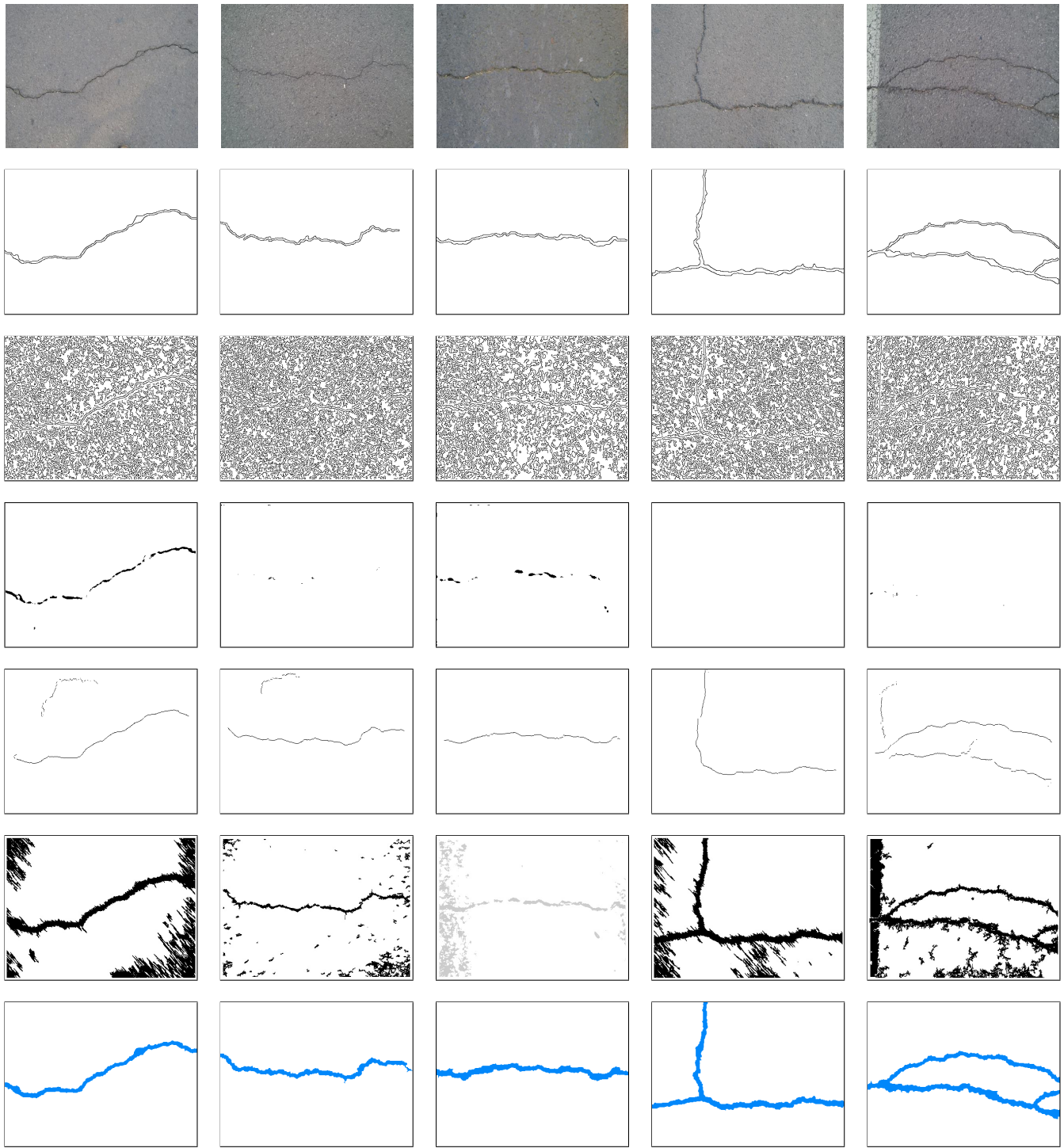
Fig. 11. Results of different algorithms on CFD (From top to bottom: original image, ground truth, Canny, CrackIT, CrackTree, FFA and CrackForest)
