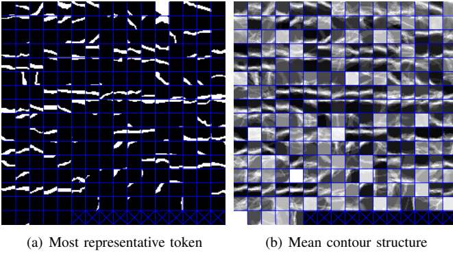
Fig. 2. Examples of tokens learned from manually labelled image database. (a) shows the most representative token for each token set. (b) shows the mean contour structure for each token set.
