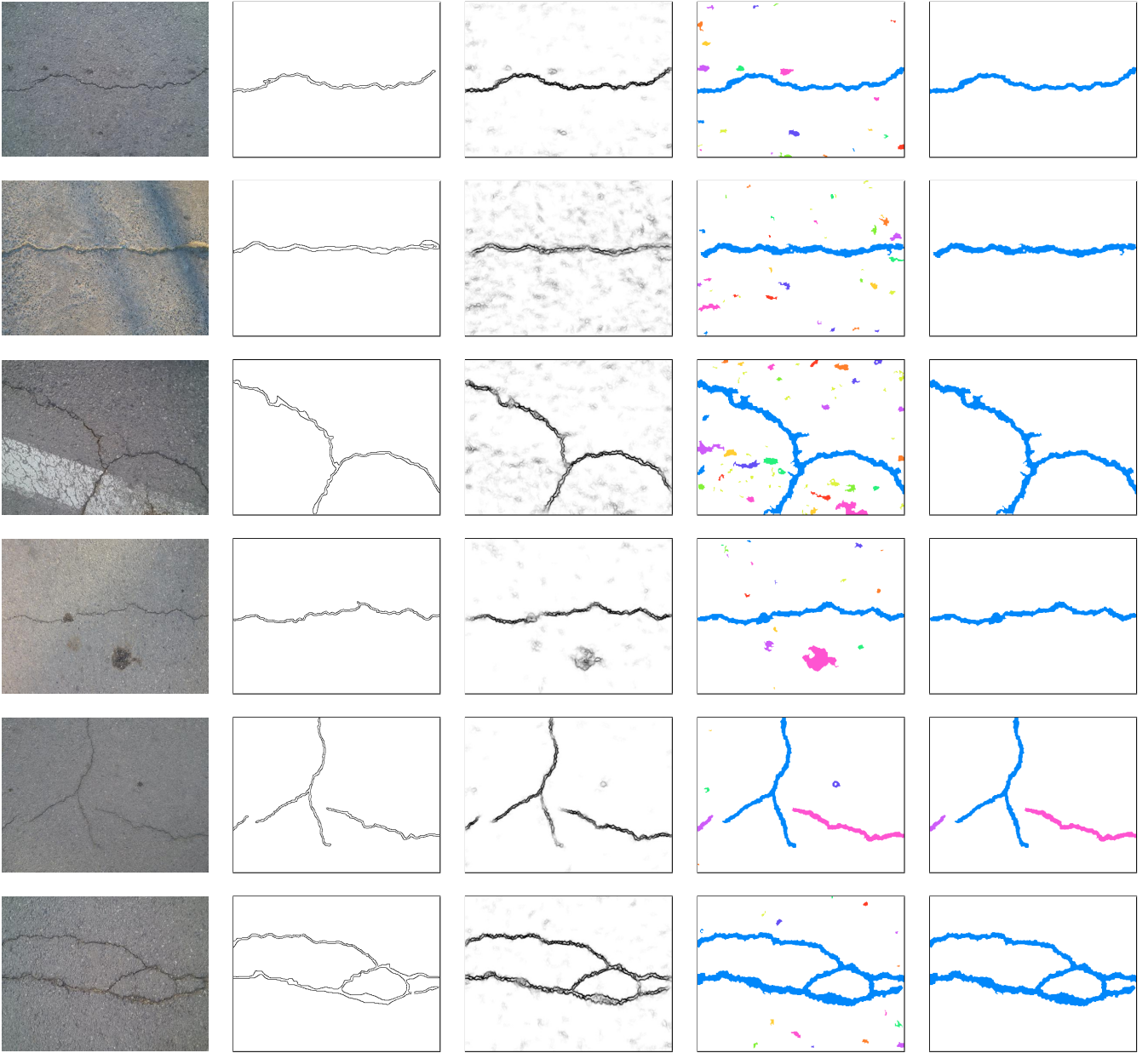
Fig. 10. Part of the results of road crack detection using our proposed method. Notice that our method can eliminate the influence of oil stains, shadows and complex background effectively, and can cope with miscellaneous crack topology.
