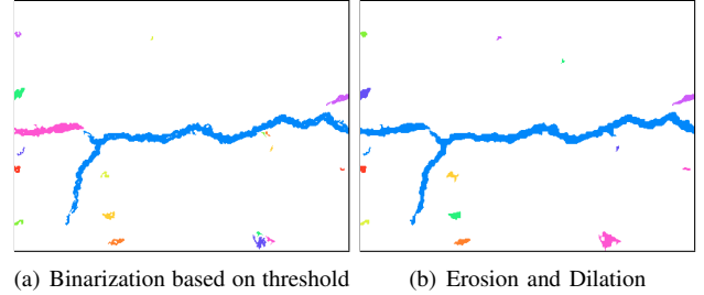
Fig. 7. (a) shows the binarization result based on threshold when \alpha = 0.1 (removing pixels of low probability according to the given probability map). (b) shows the result after erosion and dilation with a 4-by-4 rectangular structuring element.
