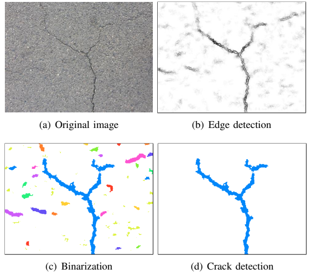
Fig. 1. Consider the pavement surface shown in image (a). (b) shows the preliminary detection results after applying random structured forests. Darker color indicates that the pixel is more likely to contain a crack. After eroding and dilating, the result is shown in (c). (d) shows the final result after the classification stage.
