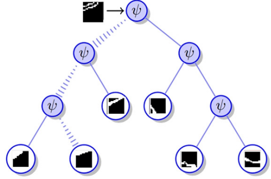
Fig. 5. The routing path of an image patch.
