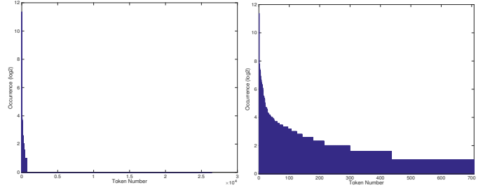
(a) The occurrence of all the tokens in descending order (b) The occurrence of the 708 most frequent tokens in descending order
